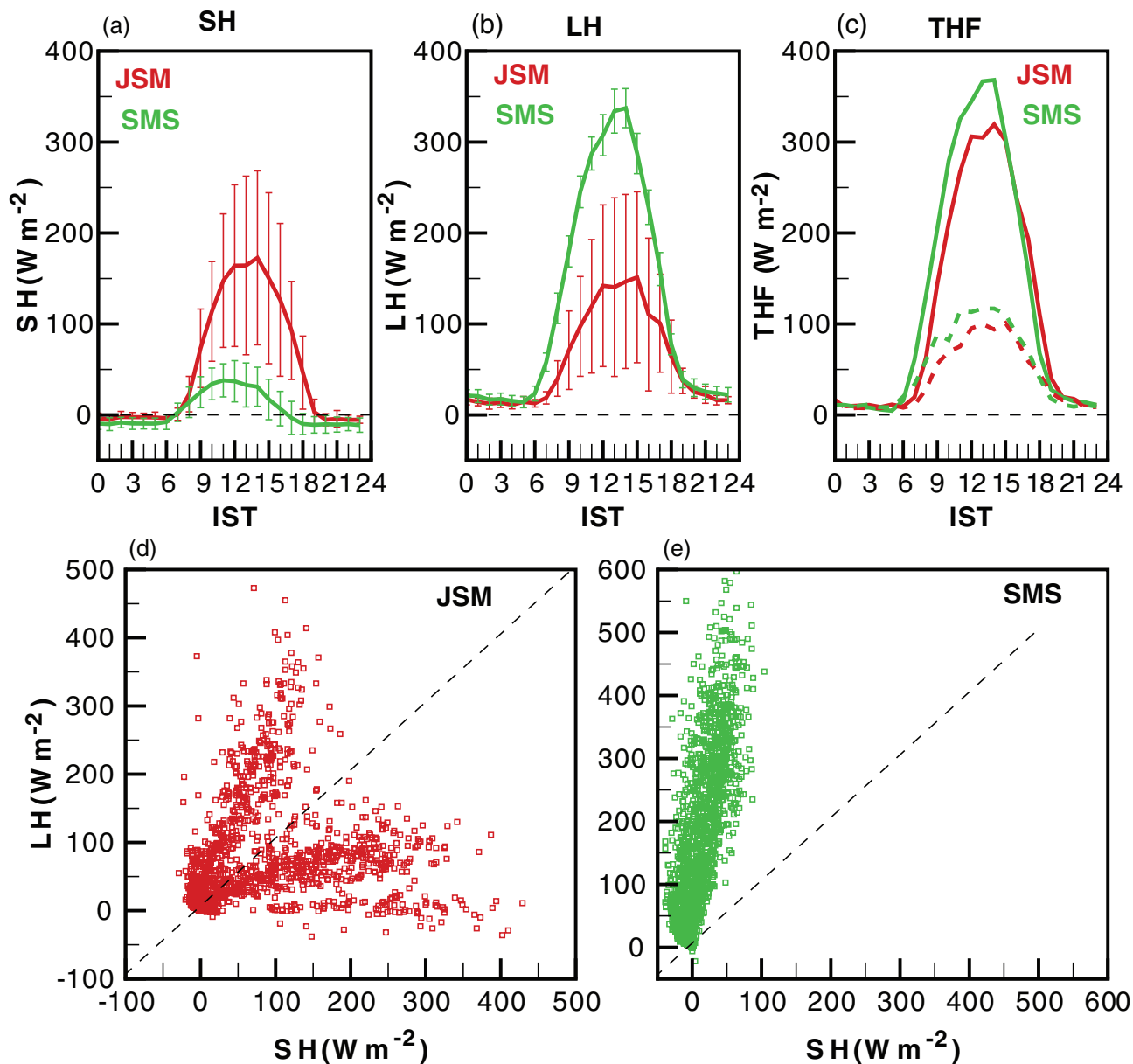
FIGURE 7 Diurnal variation of (a) sensible-heat flux (SH); (b) latent-heat flux (LH); (c) turbulent-heat flux (where THF = SH + LH ), in which red and green refer to Jaiselmer and Samastipur, respectively; (d) SH versus LH at Jaiselmer; and (e) SH versus LH at Samastipur. Data are sampled over August 2016. Day-to-day variability is quantified by one-standard deviation error bars in (a,b) or dashed lines in (c). Units are W/m^2 . The time axes in (a–c) are expressed in terms of Indian Standard Time (IST, UTC + 5 h 30 min)
