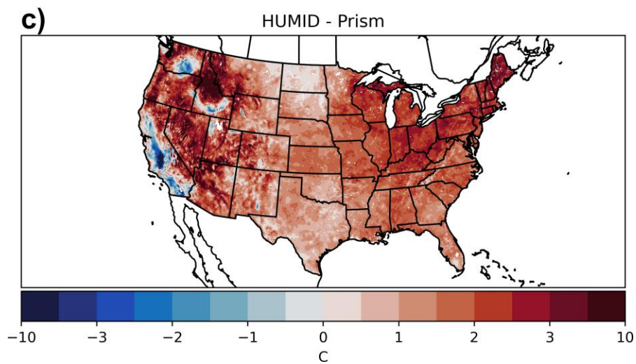
Figure S11. 1981-2017 average daily JJA Td for a) HUMID, b) PRISM, c) HUMID – PRISM.
