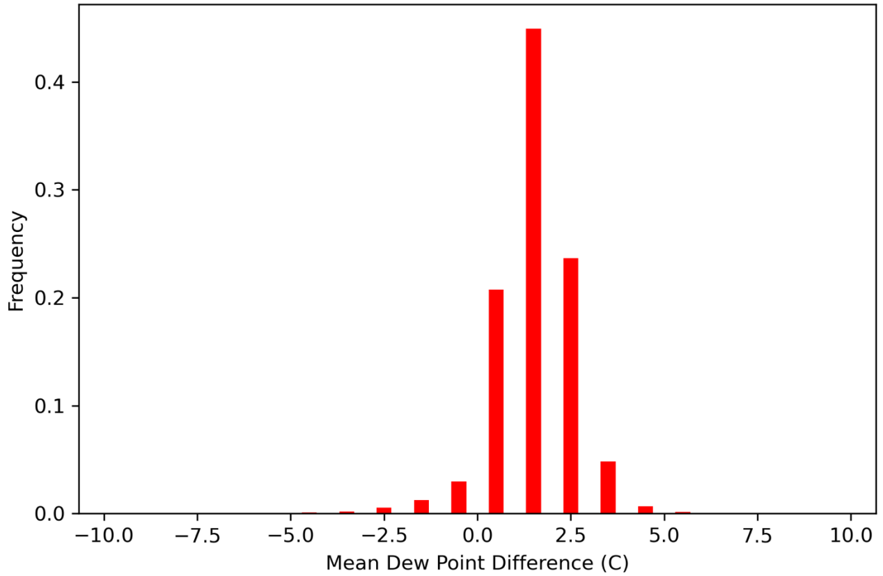
Figure S12. 1981-2017 average daily JJA Td HUMID - PRISM histogram.
