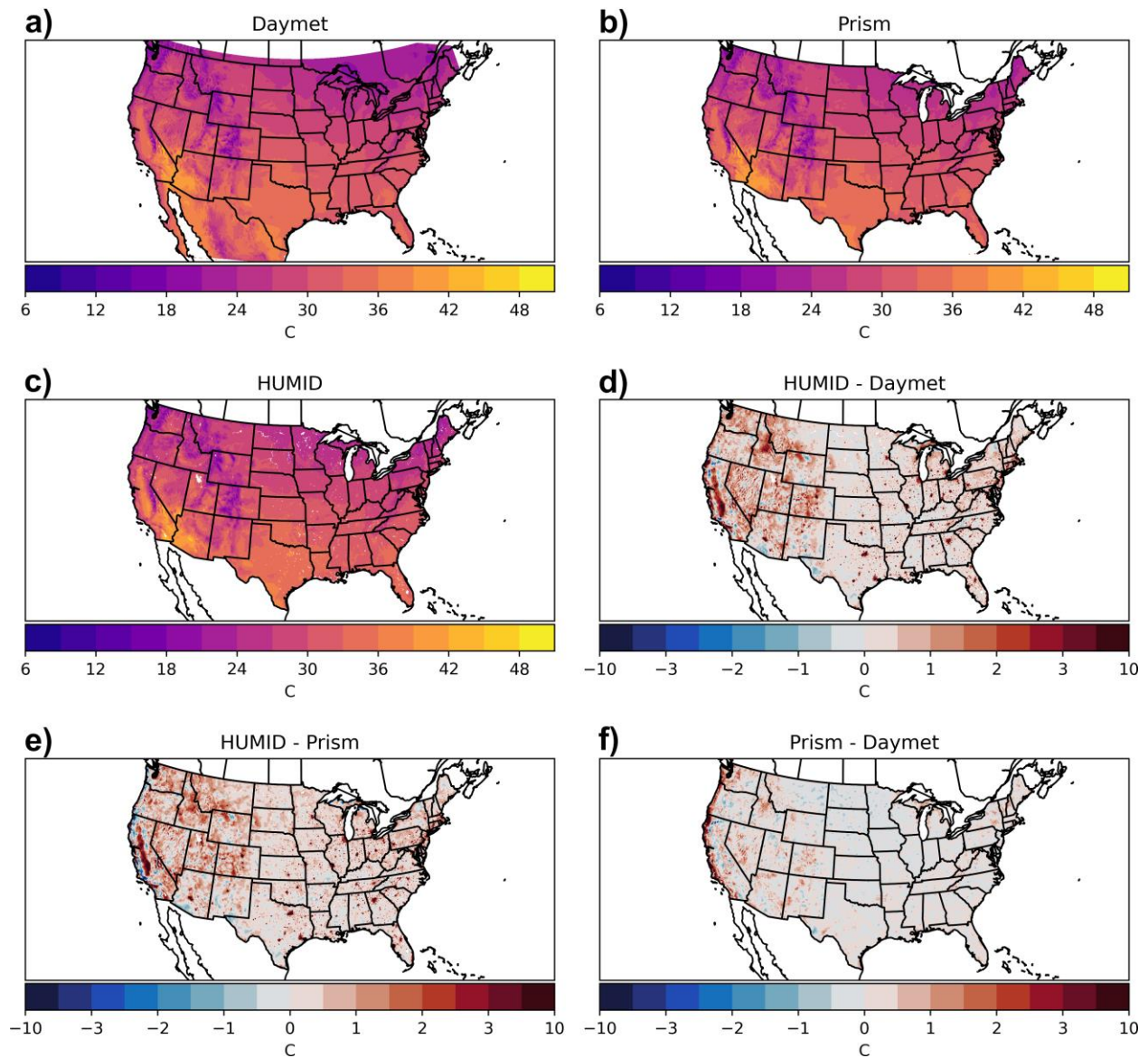
Figure S3. 1981-2017 average daily JJA Tmax for a) Daymet, b) PRISM, c) HUMID, d) HUMID – Daymet, e) HUMID – PRISM, f) PRISM – Daymet.
