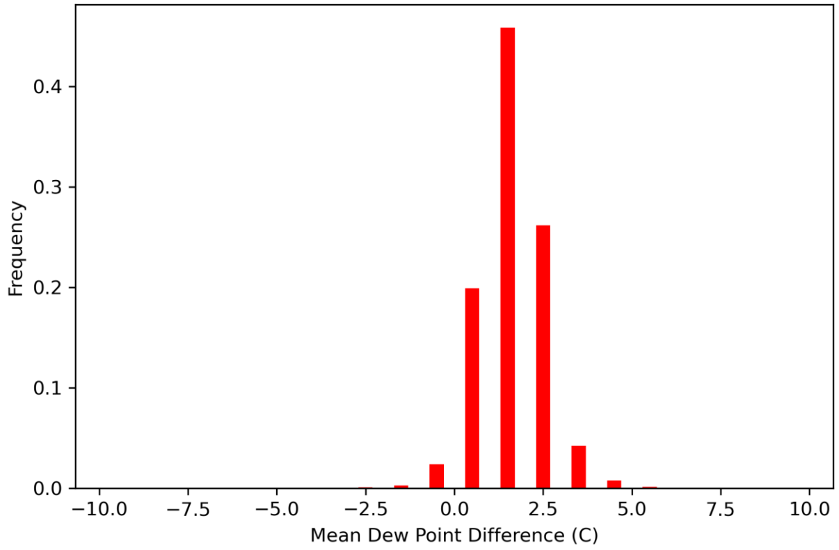
Figure S10. 1981-2017 average daily DJF Td HUMID – PRISM histogram.
