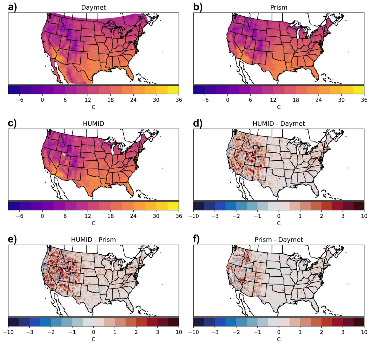
Figure S7. 1981-2017 average daily JJA T min for a) Daymet, b) PRISM, c) HUMID, d) HUMID – Daymet, e) HUMID – PRISM, f) PRISM – Daymet.
