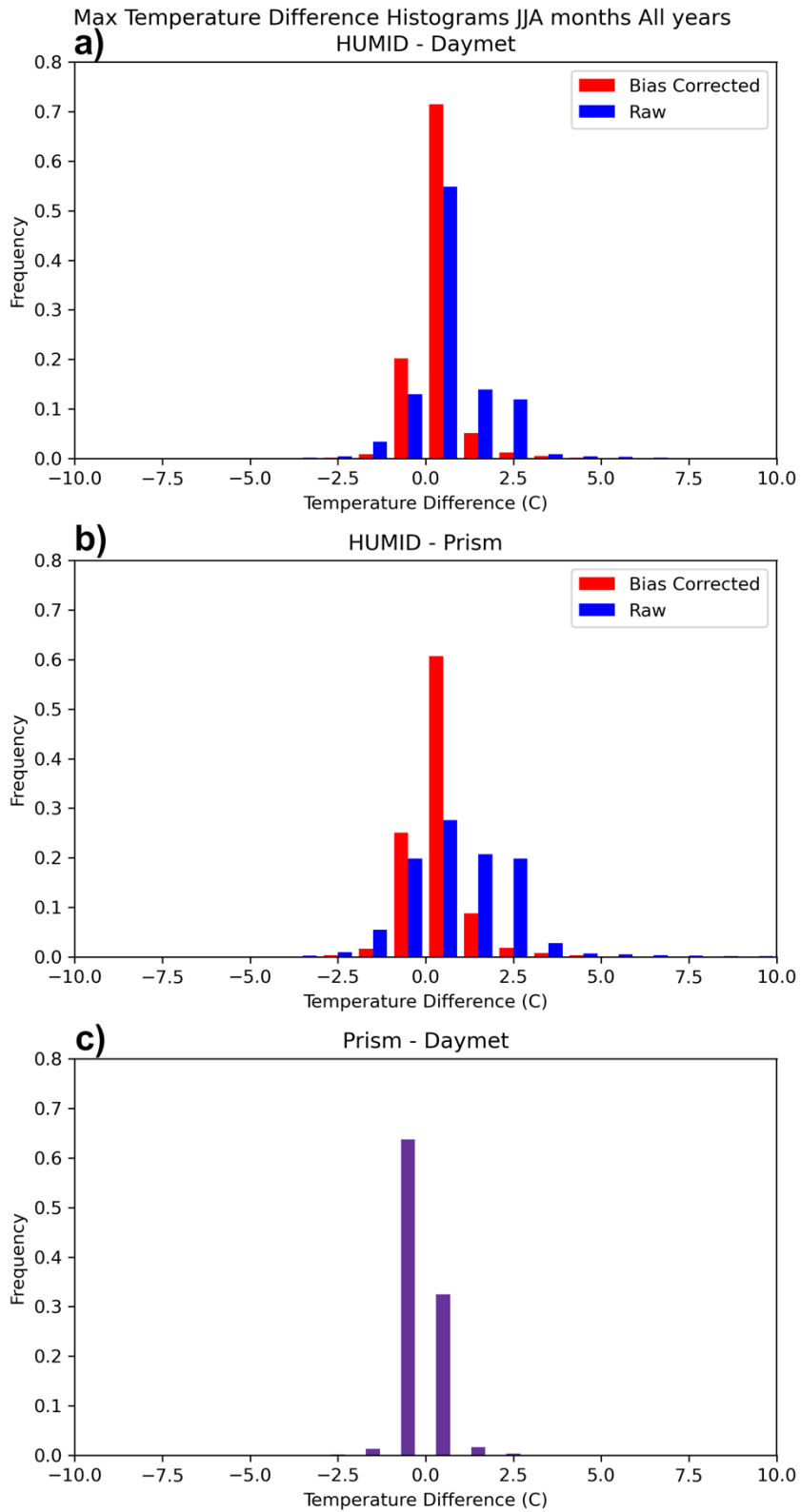
Figure S4. 1981-2017 average daily JJA Tmax difference histograms for a) HUMID - Daymet, b) HUMID - PRISM, and c) PRISM - Daymet.
