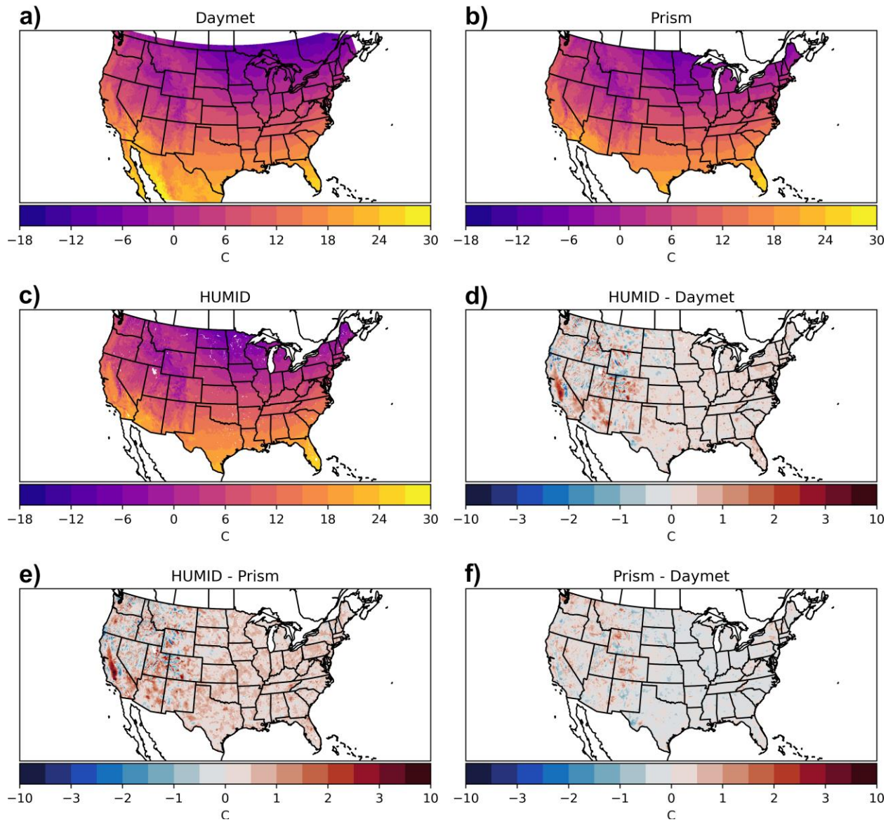
Figure S1. 1981-2017 average daily DJF Tmax for a) Daymet, b) PRISM, c) HUMID, d) HUMID - Daymet, e) HUMID - PRISM, f) PRISM - Daymet.
