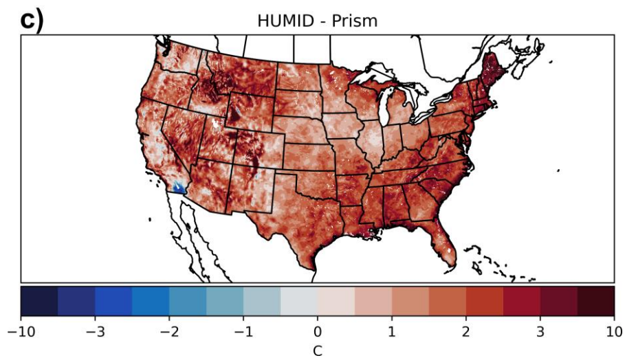
Figure S9. 1981-2017 average daily DJF Td for a) HUMID, b) PRISM, c) HUMID – PRISM.
