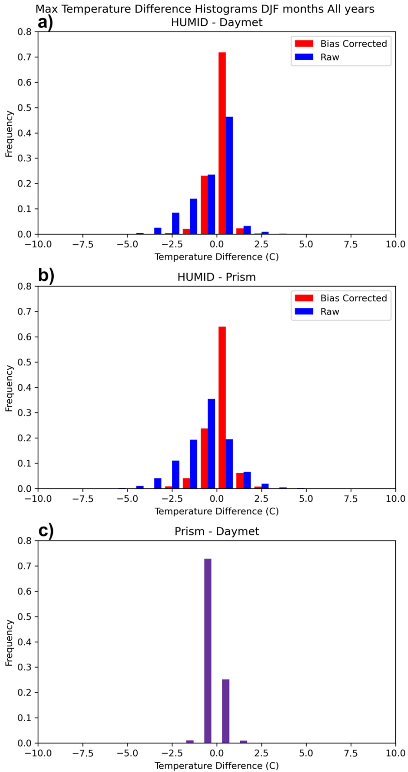
Figure S2. 1981-2017 average daily DJF Tmax difference histograms for a) HUMID - Daymet, b) HUMID - PRISM, and c) PRISM - Daymet.
