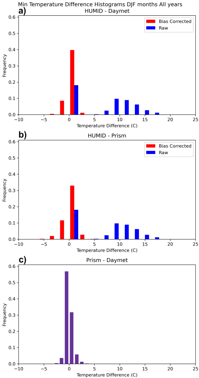
Figure S6. 1981-2017 average daily DJF Tmin difference histograms for a) HUMID - Daymet, b) HUMID - PRISM, and c) PRISM - Daymet.
