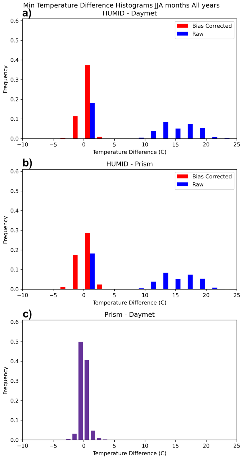
Figure S8. 1981-2017 average daily JJA Tmin difference histograms for a) HUMID - Daymet, b) HUMID - PRISM, and c) PRISM - Daymet.
