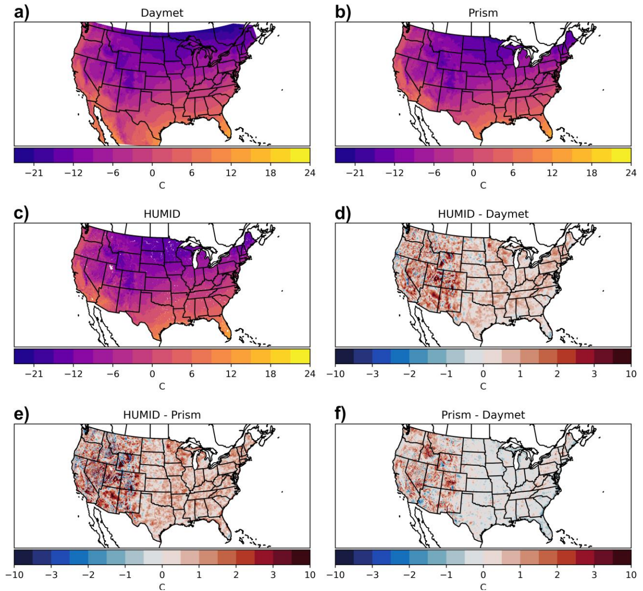
Figure S5. 1981-2017 average daily DJF Tmin for a) Daymet, b) PRISM, c) HUMID, d) HUMID - Daymet, e) HUMID - PRISM, f) PRISM - Daymet.
